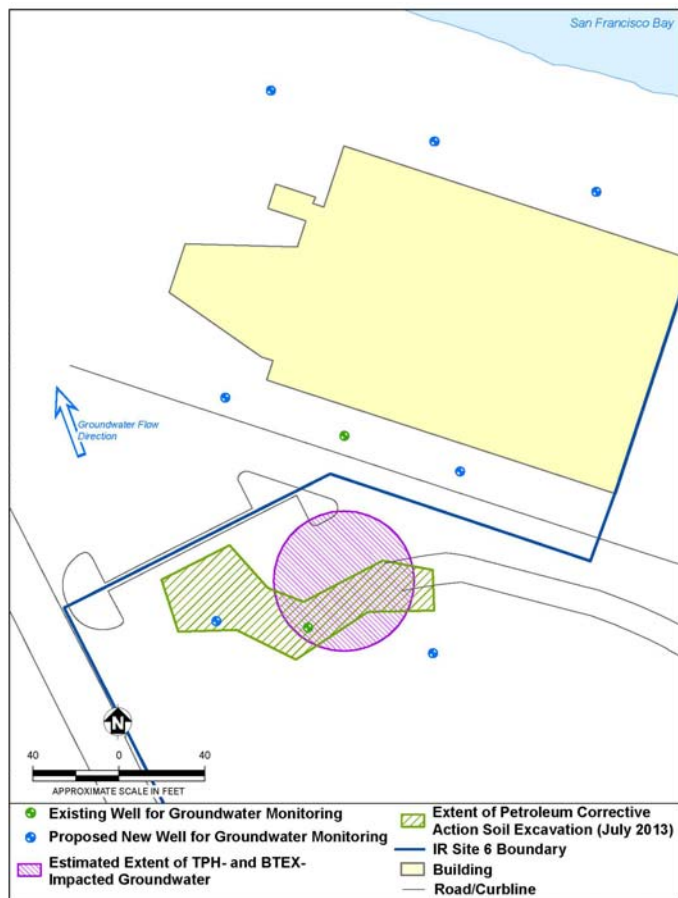
Figure 7. Alternative GW-2 – ICs and Groundwater Monitoring
