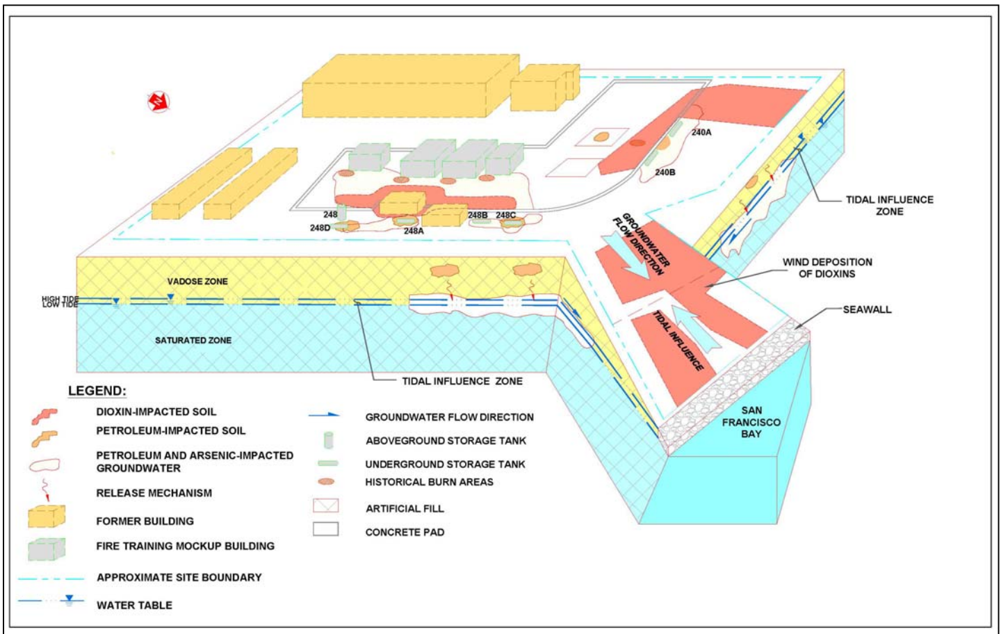
Figure 4. Conceptual Site Model for Site 6
