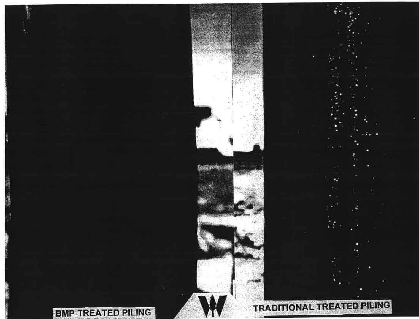
Fig. 2. A new pile treated with creosote to BMP standards, prior to weathering, compared to a pile treated to traditional standards. Note the obvious residual surface creosote on the pile receiving the traditional treatment. (Photo courtesy of R. D. Hayward.)
