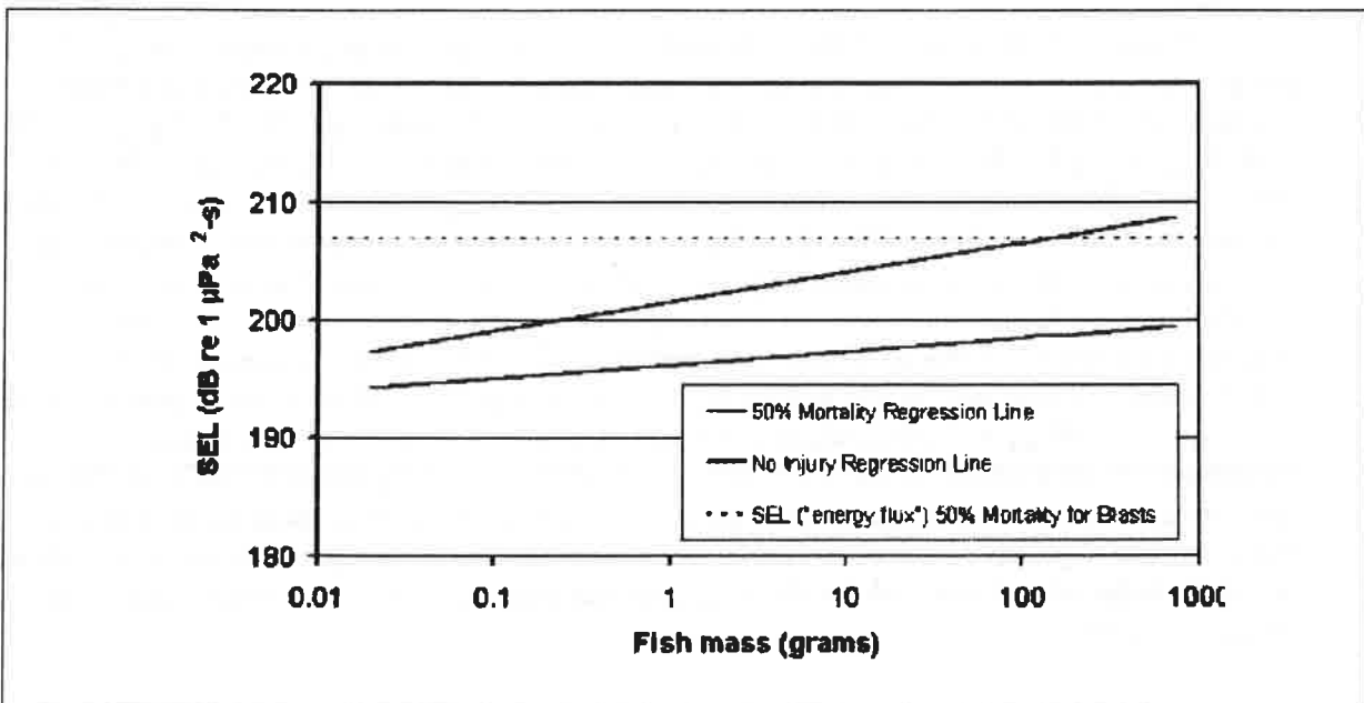
Figure B2: Comparison of lethal energy flux reported in the literature with the recommended guidance for physical injury and 50% mortality. Both are derived from explosive blast effects data on fish and therefore should be conservative for exposure to a single pile driving impact.
