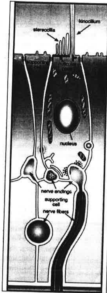
Figure 4. Schematic drawing of a sensory hair cell from a fish. The transducing element is the ciliary bundle, made up of the kinocilium and stereocilia, at the apical (top) end of the cell. This bundle is in contact with the otolith that lies in the chambers of the otolithic end organs (sacculle, lagena, utricle). Relative motion between the sensory cell body sitting in the sensory epithelium and the overlying otolith results in a shearing or bending of the ciliary bundle. This causes channels (sub-microscopic holes) to open in the cilia and allowing the entry of calcium ions into the cell. This results in a cascade of events that leads to the release of chemical neurotransmitters from the base of the cell. The neurotransmitter crosses a small gap between cells and excites the endings of the nerve that innervates the cell. This, in turn, results in an electrical potential (the action potential) in the nerve that is carried to the brain. (From Popper and Coombs 1980)
