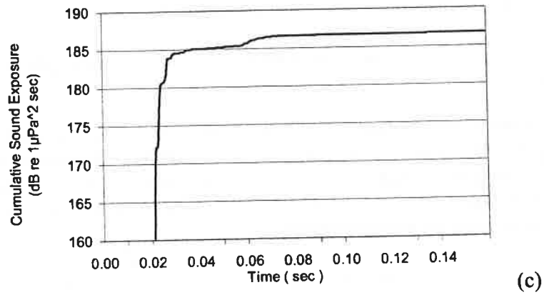
Figure 1: Measures of unattenuated pile driving sound at the San Francisco-Oakland Bay Bridge East Span Replacement project (SFOBB), Pier 3E at 50 m in relatively deep water. (a) Measured sound pressure waveform; (b) narrow-band frequency content of the waveform; (c) cumulative sound exposure (or sound pressure squared) over time. The sound exposure level (SEL) for this single hammer strike is 187 dB re 1 \mu\text{Pa}^2\text{-s} and RMS (impulse) is 200 dB re 1 \mu\text{Pa} (based on 0.048 s pulse width). Data provided by J. Reyff, Illingworth & Rodkin, Inc.
