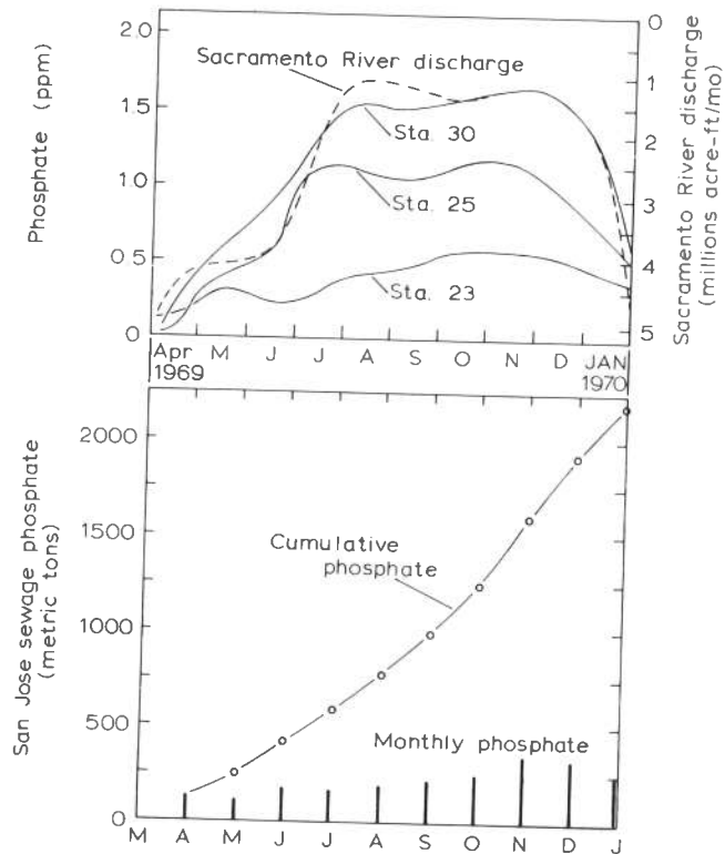
Figure 14.—Upper, Seasonal phosphate changes at three south bay stations and the Sacramento River discharge (the latter is plotted with discharge increasing downward). Lower, The amount of phosphate (metric tons) contributed each month (shown as the monthly phosphate) and the cumulative amount) to the south bay from the San Jose city sewage plant. 34
