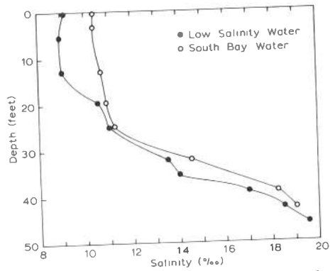
Figure 9.—Measurements of the salinity made in front of, and just behind, the edge of the low salinity flow. Note that the low salinity water is clearly distinct from the south bay water to a depth of about 20 feet.
