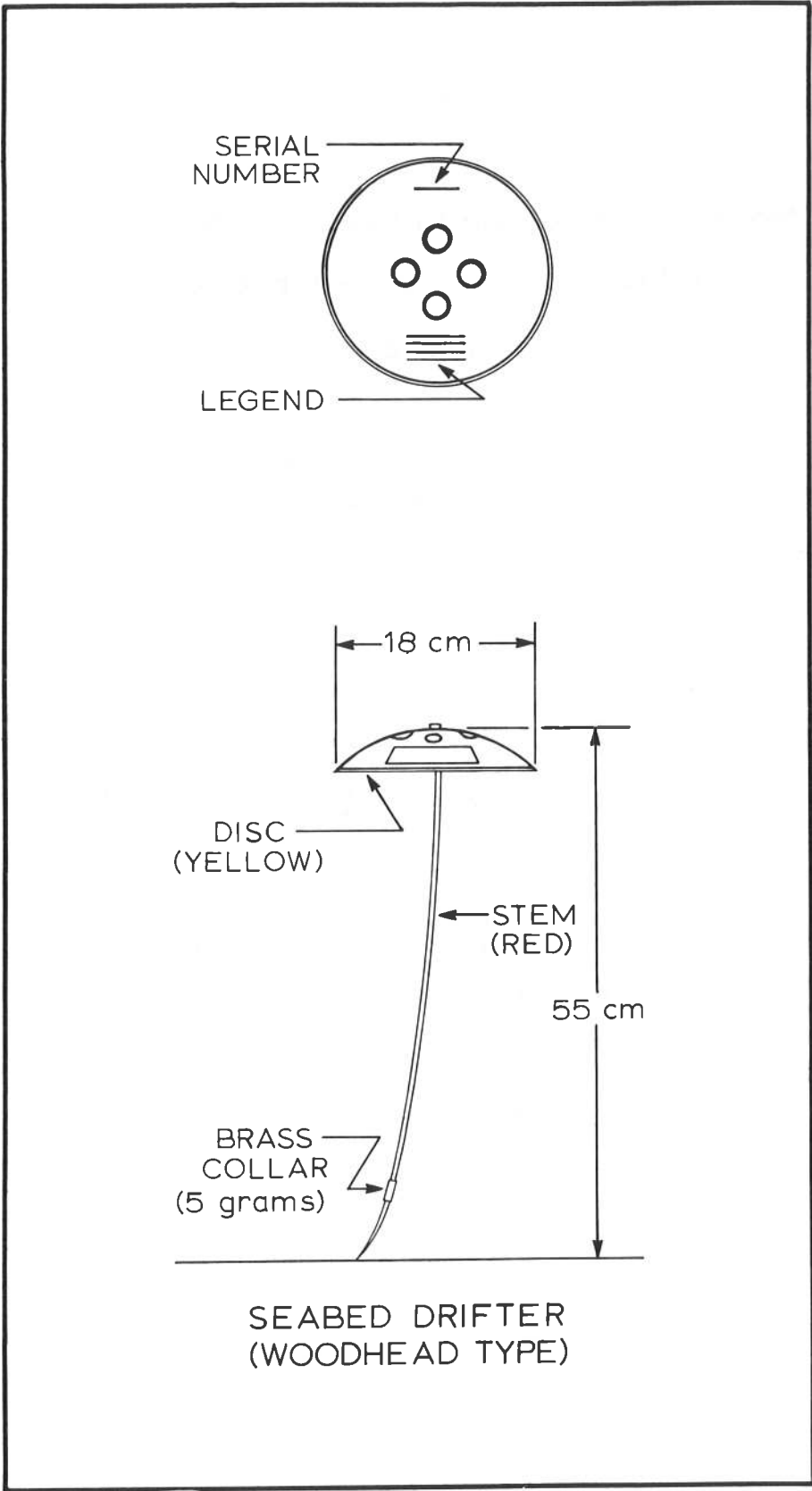
Figure 1.—Side and top view of seabed drifter. Modified from a drawing by J. B. Zocchi.
