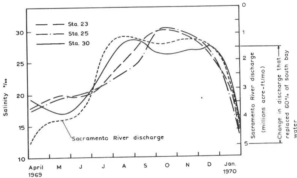
Figure 12.—Seasonal salinity changes at three south bay stations, and the Sacramento River discharge (the latter is shown with discharge increasing downward). Note the general correspondence between the changes in salinity and the discharge.
