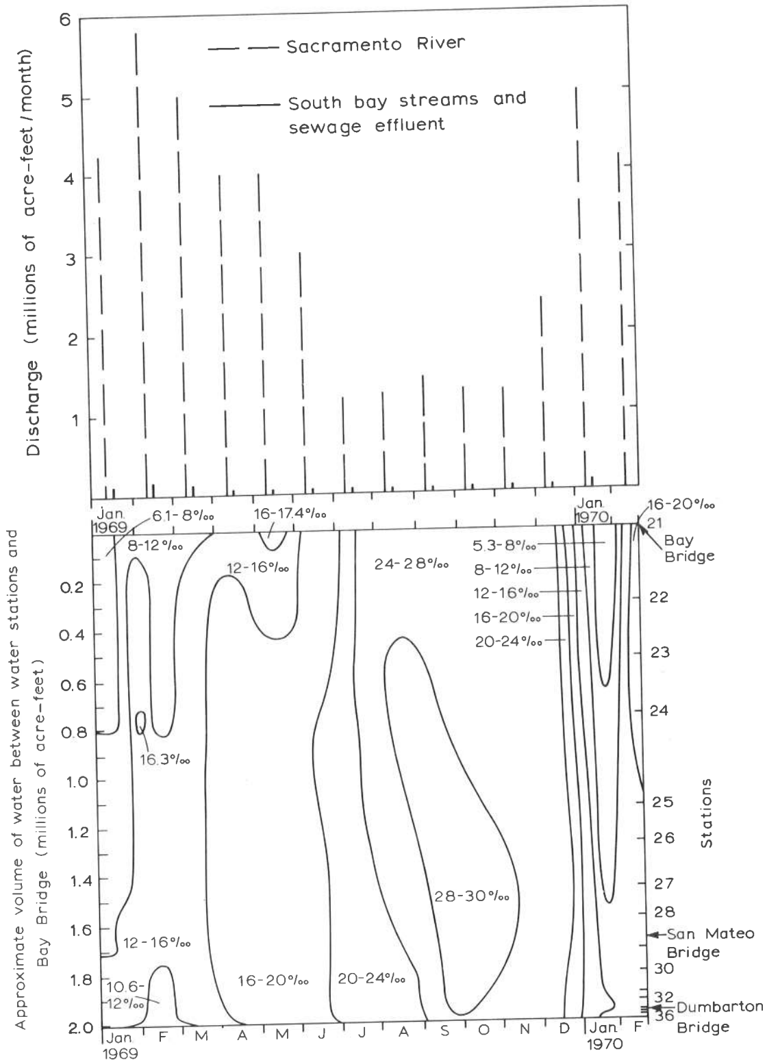
Figure 3.—The total monthly discharge of the Sacramento River and the south bay streams and sewage effluent 5, 12 upper, and the corresponding changes in the surface salinity distribution in the south bay, lower. The water-sampling stations are shown on the right in terms of the volume of water that lies between the station and the Oakland Bay Bridge. 15
